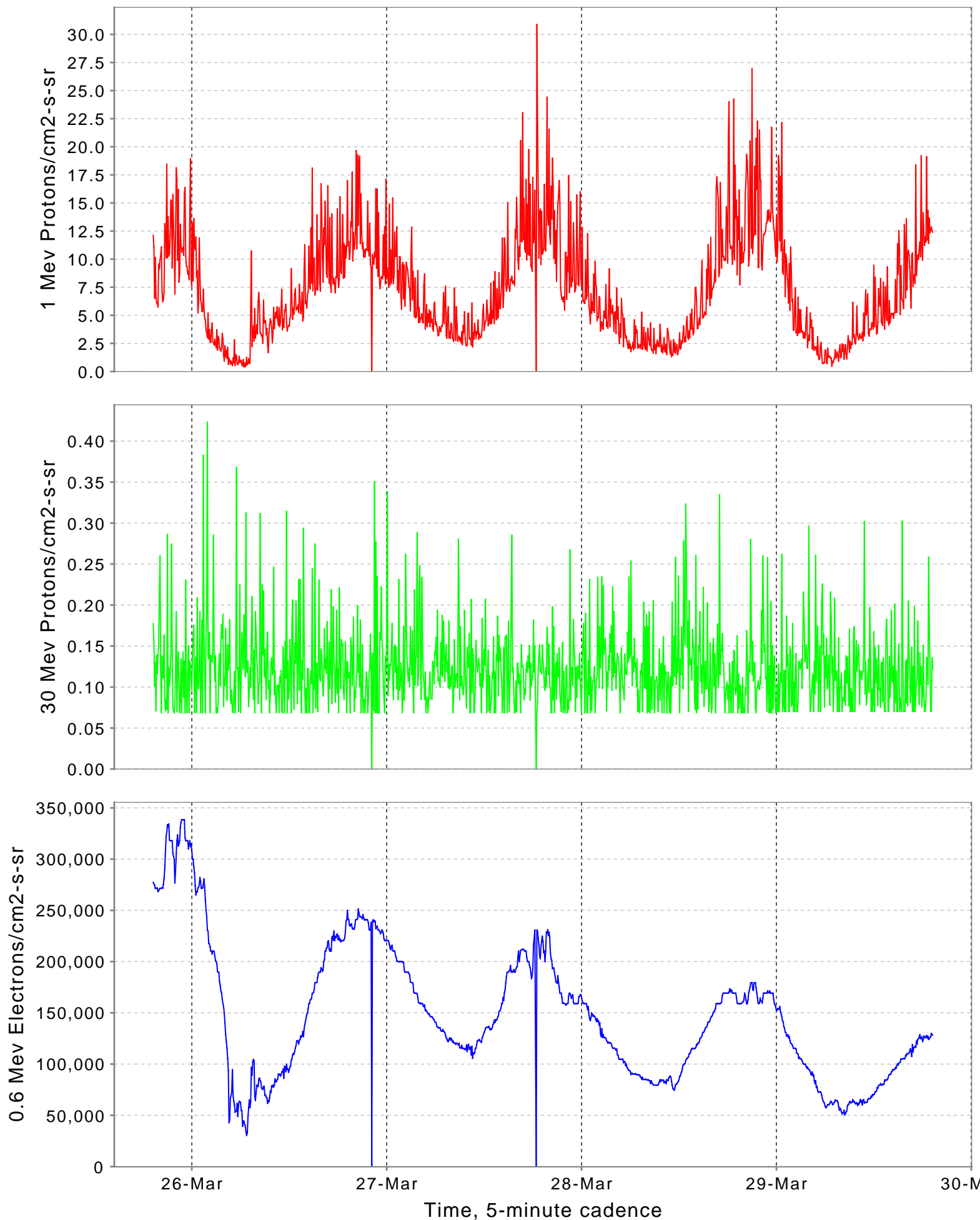
— Proton flux > 1 Mev, GOES-11 at: 135W — Proton flux > 30 Mev, GOES-11 at: 135W — Electron flux > 0.6 Mev, Ending Time: 03/29/2009 19:15
