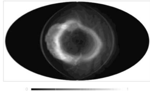
Fig. 2. Heliospheric imager synthetic product for May 29, 2003, T=10 UT derived from the HAF solar wind model. This is an example of CMEs that are tracked and used by HAF. The occulted Sun is at the center of the image.
