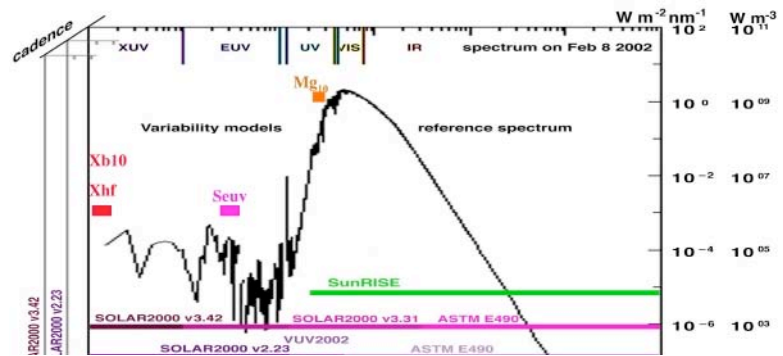
Fig. 5. The SOLAR2000 model provides irradiances and indices across the entire solar spectrum from X-rays to infrared with a daily, hourly, minutely cadences. The Mg_{10} and S_{EUV} indices are used in the Jacchia–Bowman thermospheric density model.
