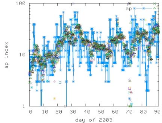
Fig. 4. ap forecast in 2003 derived from the HAF solar wind model (symbols of various shapes except asterisks) versus the actual ap (3-hour planetary geomagnetic index) (asterisks).
